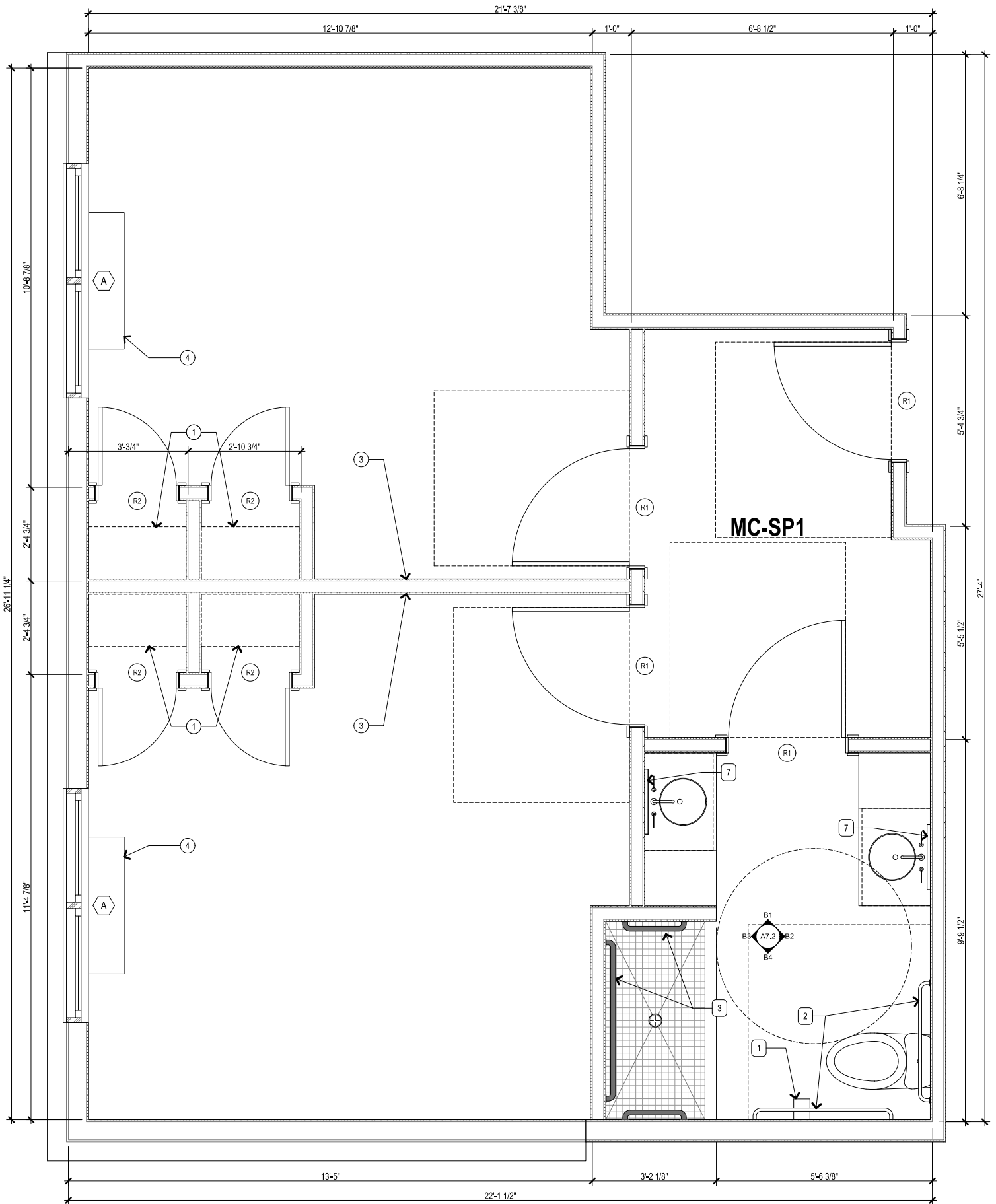
C1 TYP. MC-SP1 SCALE: 1/2" = 1'-0"
